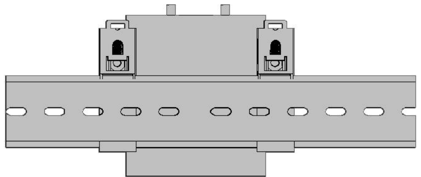
Rail mounting
