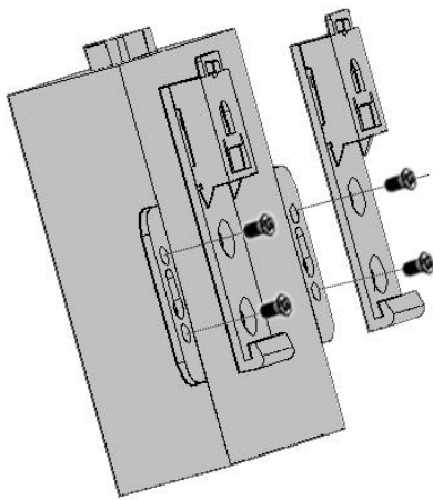
Buckle installation
